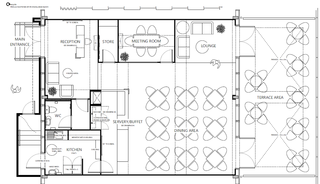
PLAN - NOMINAL SIZE - 10m x 12m - 120m 2 + TERRACE
